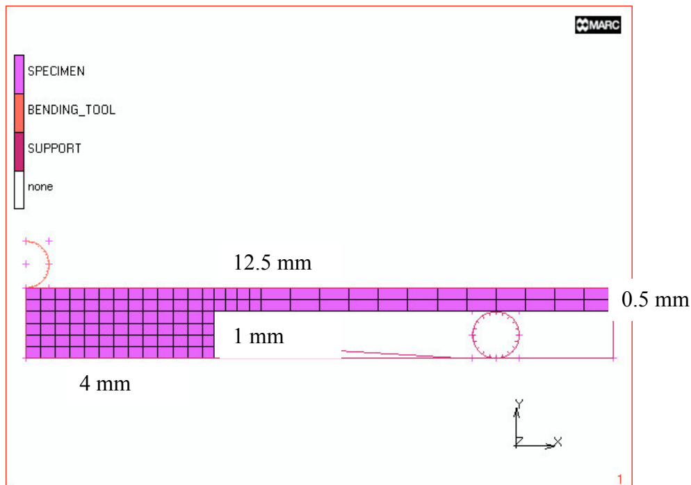
Figure 3.: Probe design using finite elements method software.
